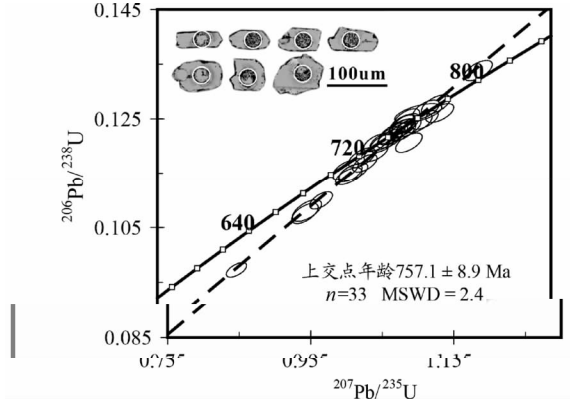
5 U-Pb AKS01 BSE Fig. 5 BSE photo and U-Pb concordia diagram of zircons from the mafic dyke AKS01 intruding the Aksu blueschists
